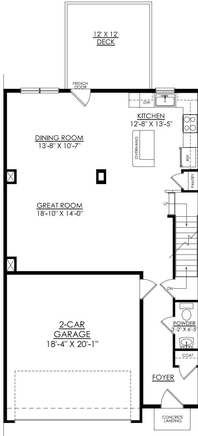
○ FIRST FLOOR PLAN CC- MID UNIT
