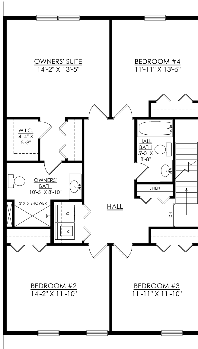
○ SECOND FLOOR PLAN CC- MID UNIT
